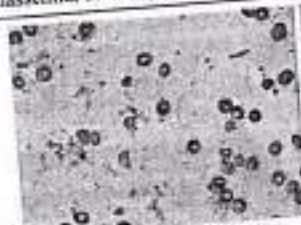
Fig 3:- Showing Schistocytes
